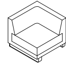
end sofa w750 x d750 x h720; sh 380
