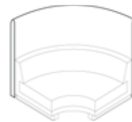
curved screen 1125 radius x d65 x h1250
